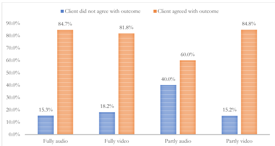
Figure 26: Client agreement with outcome by mode of hearing
